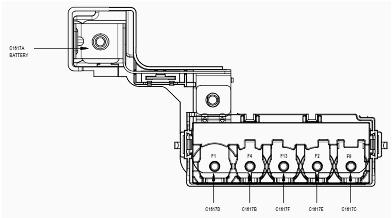
High Current Battery Junction Box (BJB)
