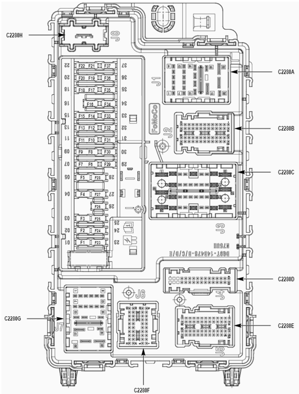
Body Control Module (BCM)
