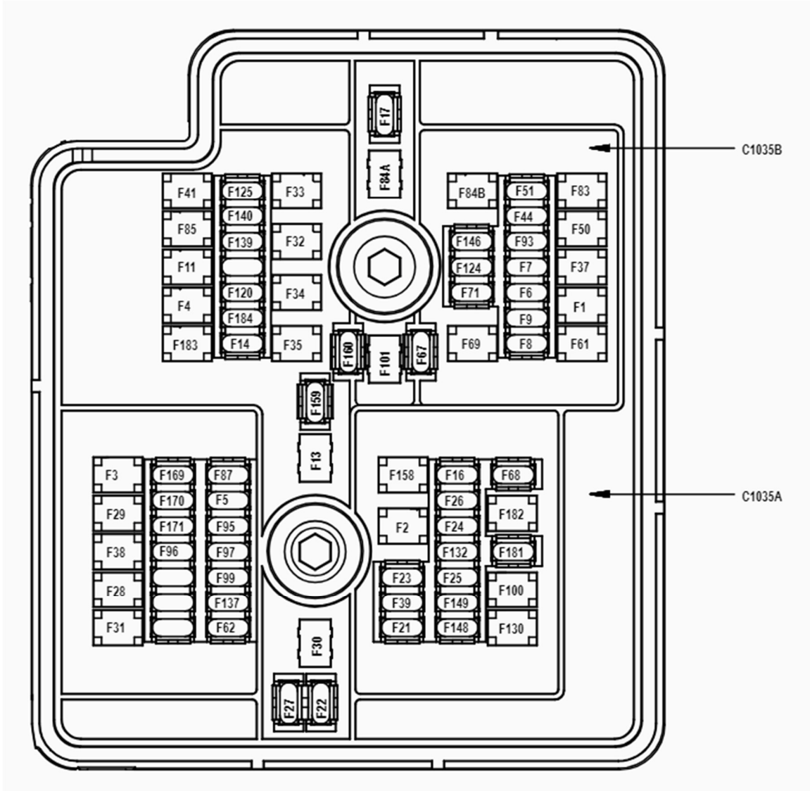
Battery Junction Box (BJB)
