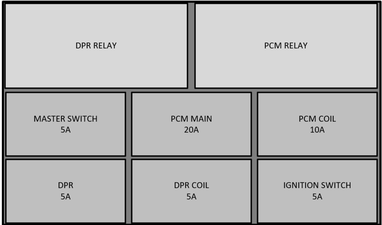
PCM/Diff Pump Fuse Box
