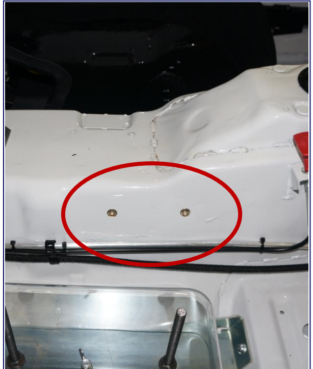
Radio Mounting Location (2) M6 Rivnuts Provided
