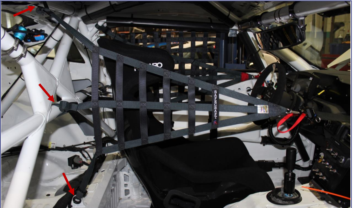
RH Helmet Support Net (Ratchet Release) Mounting Points
