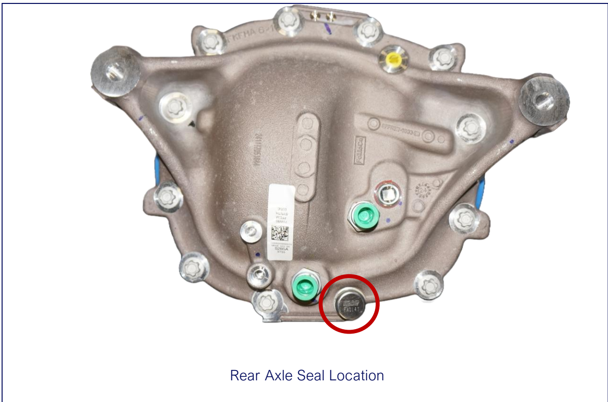
Sealed Rear Axle 3.55 (REQUIRED) FP-4001-DHRA
