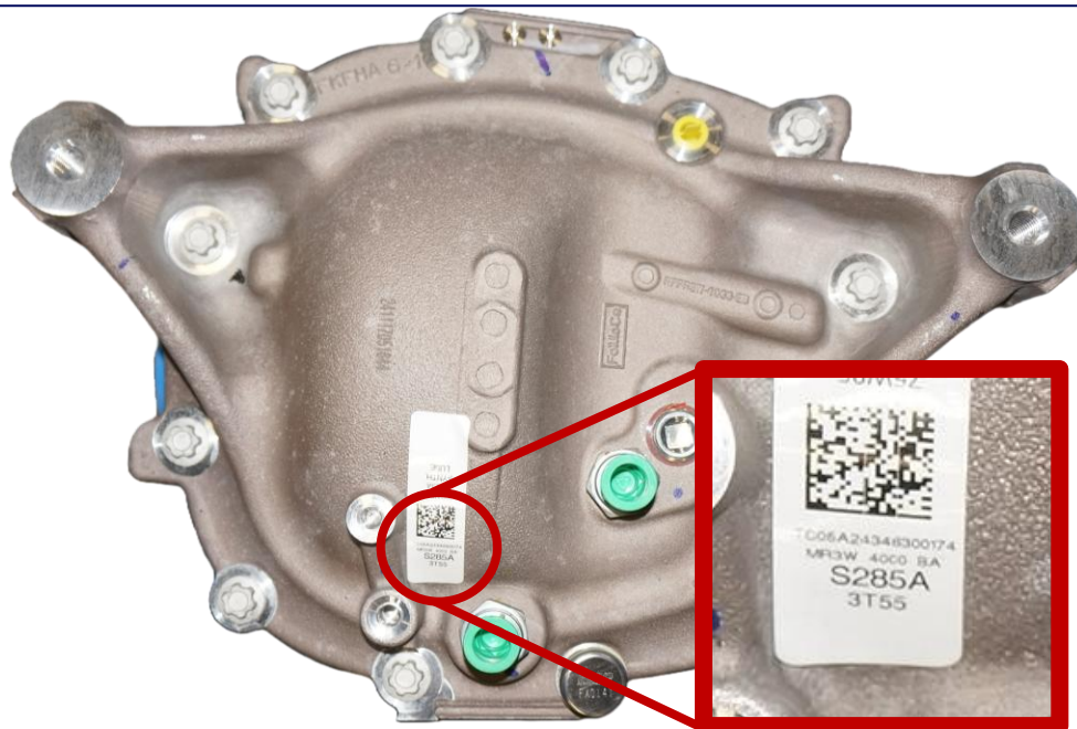
Sealed Rear Axle 3.55 (REQUIRED) FP-4001-DHRA
