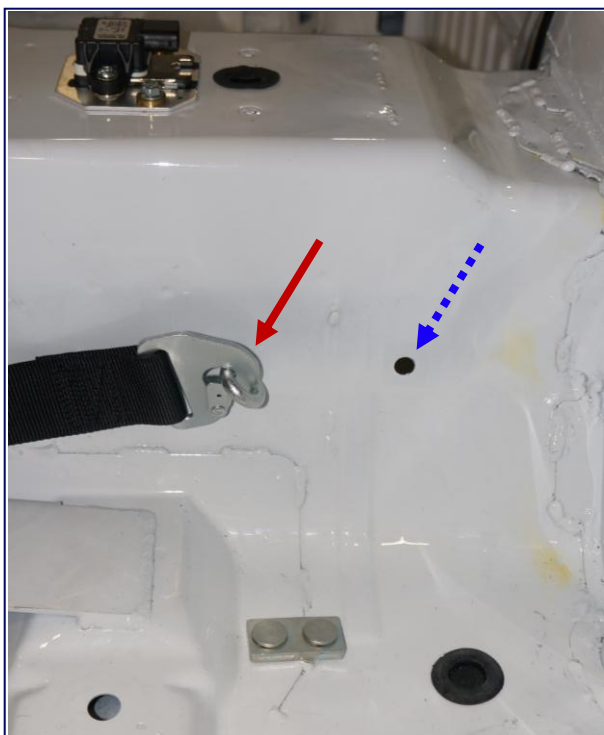
Standard Harness Mount Location (Red) Optional Harness Mount Location for use with Inboard Seat Mount Location (Blue Dashed) Left Side of Drive Shaft Tunnel
