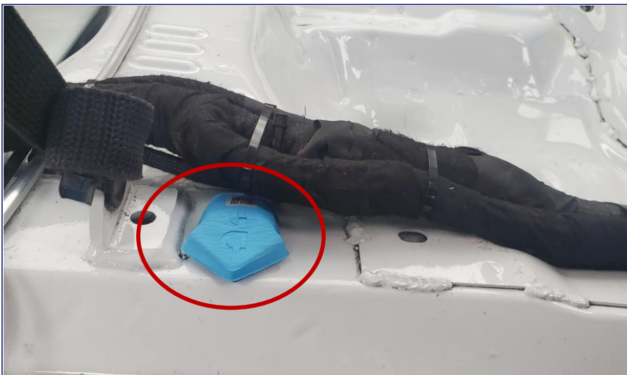
Incident Data Recorder Location Rear Seat "Shelf" on Centerline
