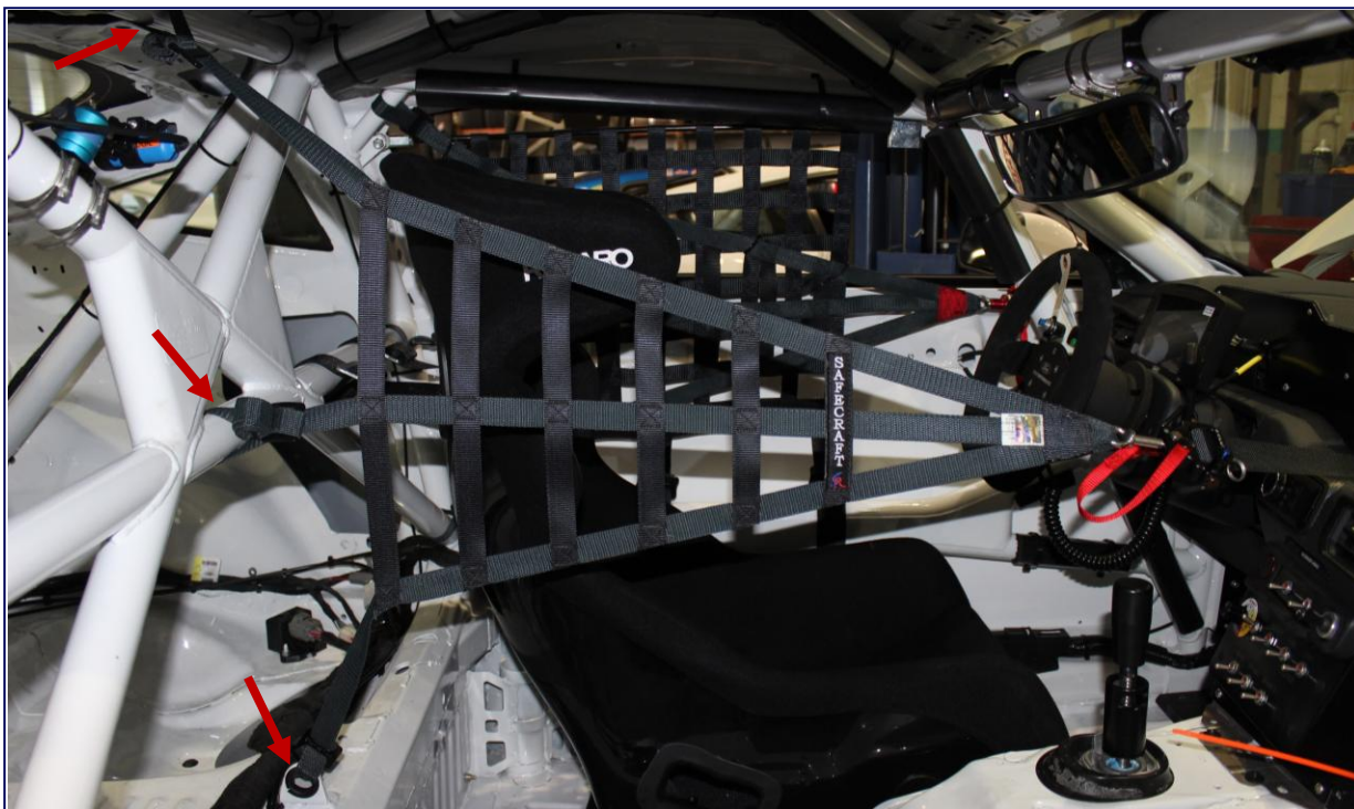
RH Helmet Support Net (Ratchet Release) Mounting Points
