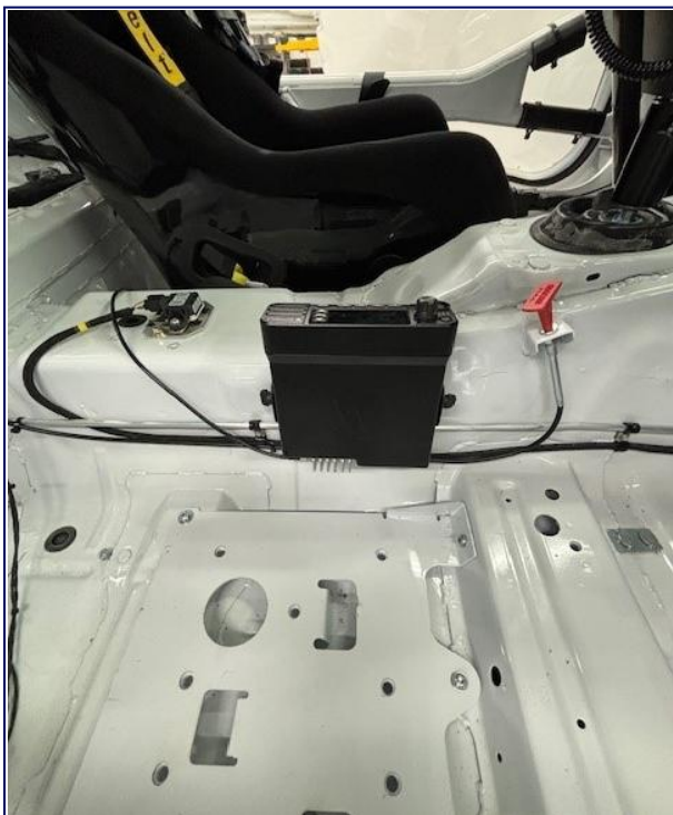
Radio Location Right Side of Drive Shaft Tunnel
