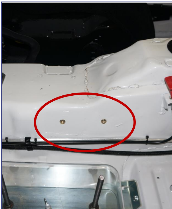
Radio Mounting Location (2) M6 Rivnuts Provided
