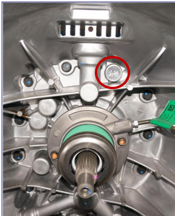
Transmission Seal Location 2 Inside Bell Housing
