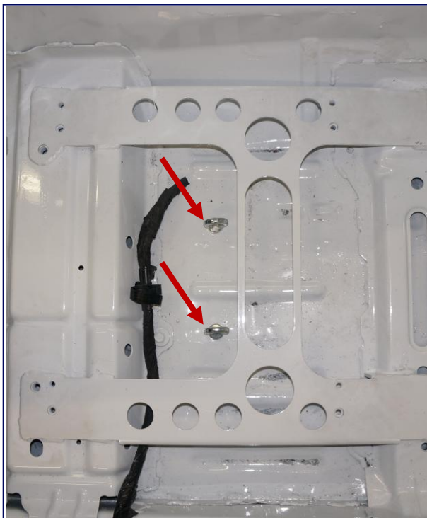
Harness Mounting Points Driver's Side Floor
