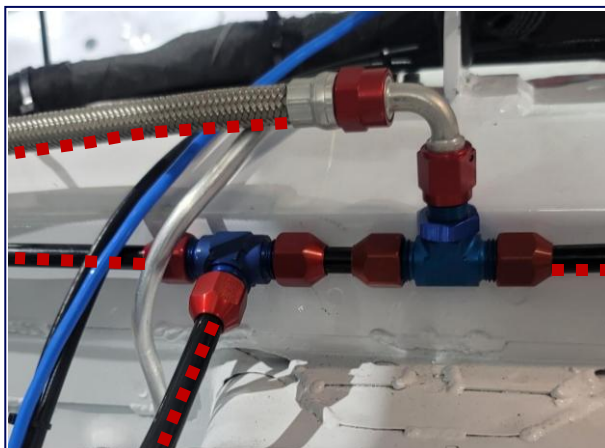
Airline Union to Rear Air Jacks / Air Feed Line Junction
