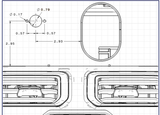
Panel Cut Diagram for Light (all dimensions are in inches)
